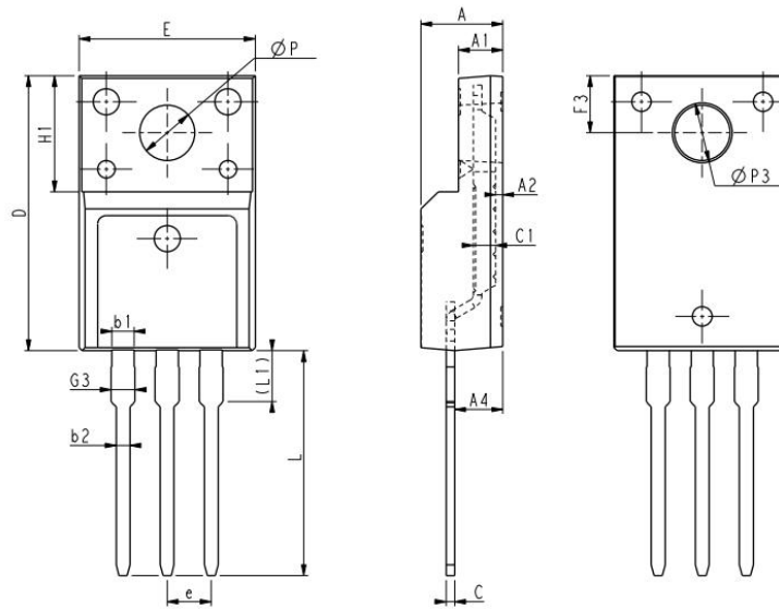
COMMON DIMENSIONS
